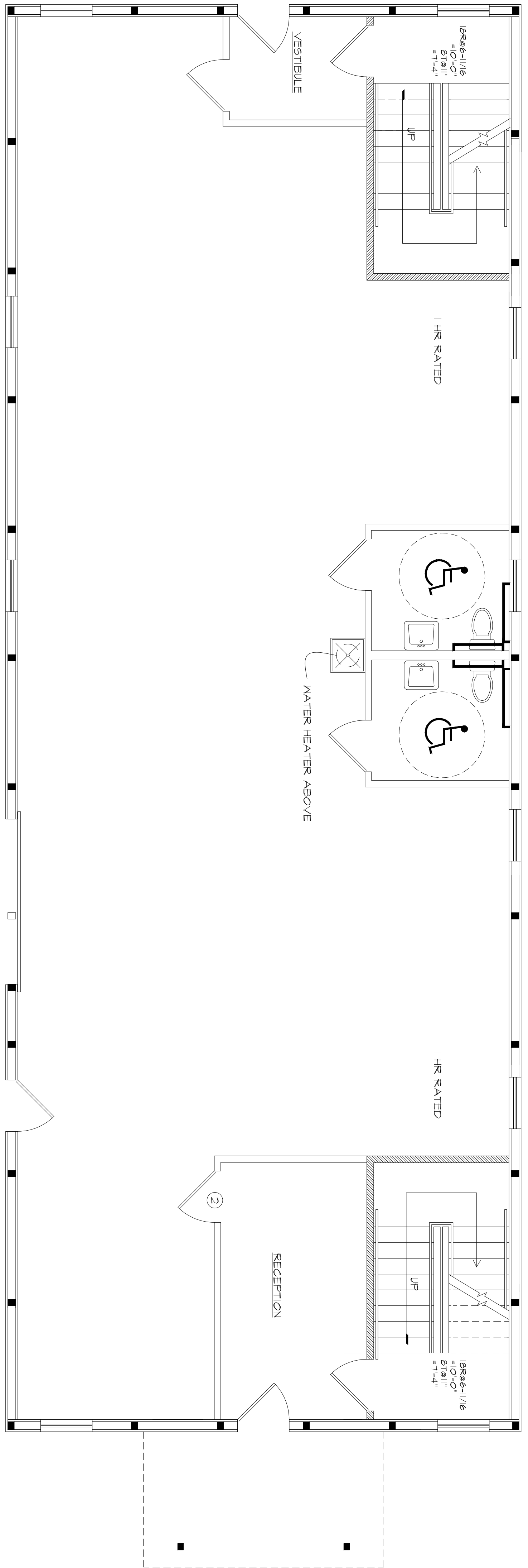
FIRST FLOOR PLAN 1/2" = 1'-0"
